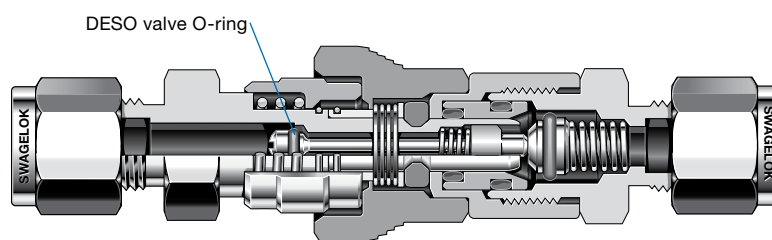
Double-End Shutoff (DESO)—Red Stem Sleeve
